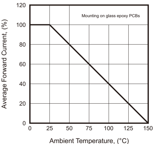
Fig.4 - Current Derating Curves
